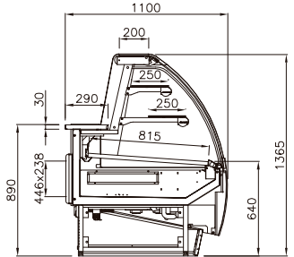
PAPN neutral neutral neutra neutra
